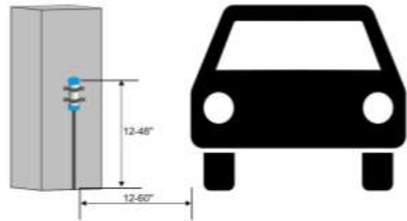
Above-Grade Installation
