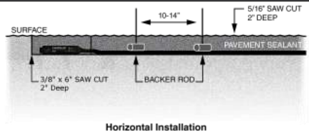
Horizontal Installation
