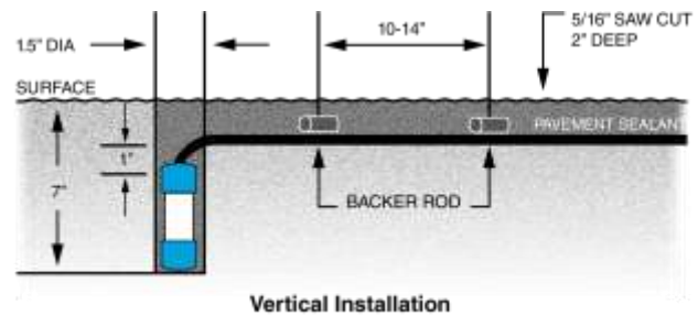
Vertical Installation
