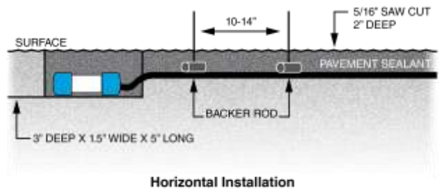
Horizontal Installation
